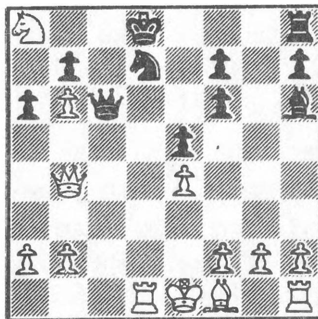
408 After 17...Kd8
